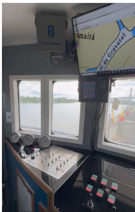
Figura 2.6.1-4: Painel de Controle - Draga SC Dredger
